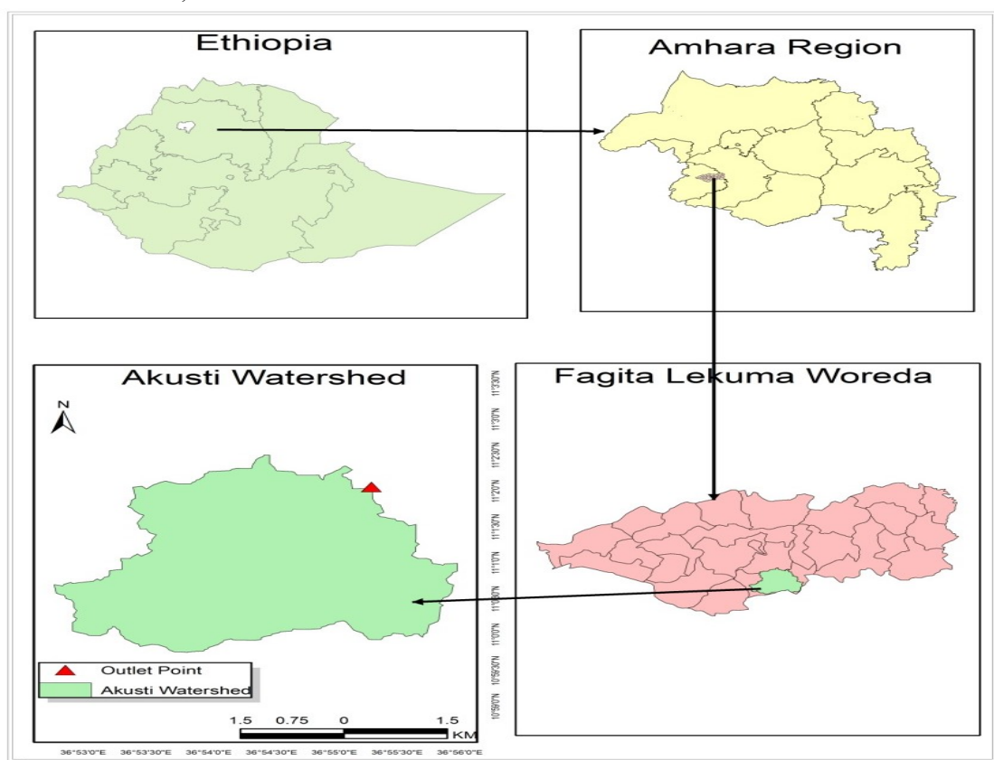
Figure 1. Location map of Akusiti watershed
