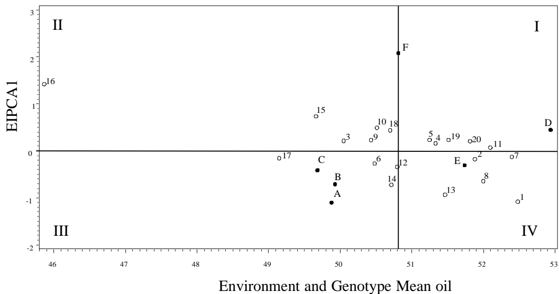
Figure 2. Biplot of IPCA1 against both genotype and environmental mean
