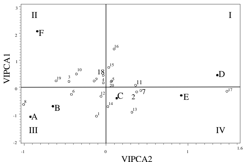
Figure 3. Biplot of IPCA1 against IPCA2 for both genotypes and environments
